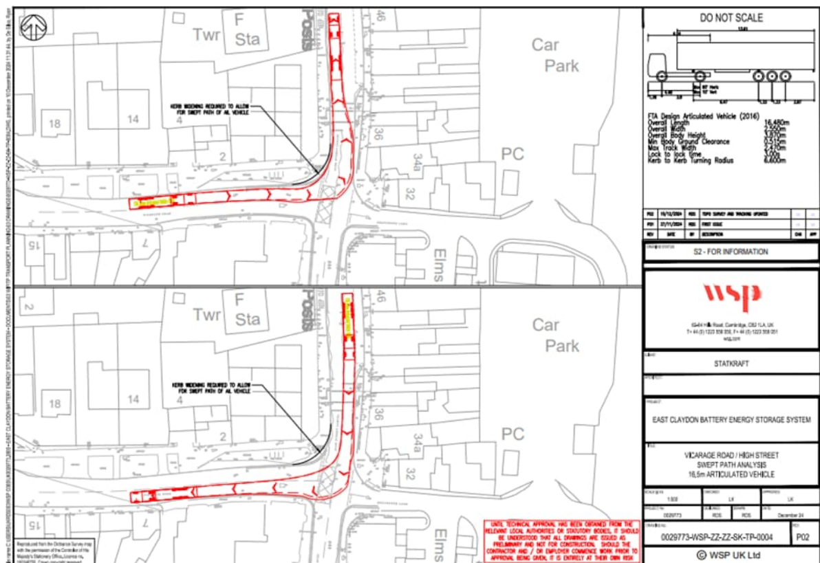
Figure 4: Swept Path Assessment Plan
